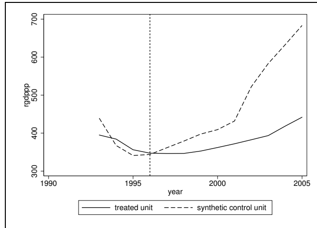
Figure 16. Trends in Real GDP Per Capita, Uzbekistan vs. Synthetic Control - Case A
